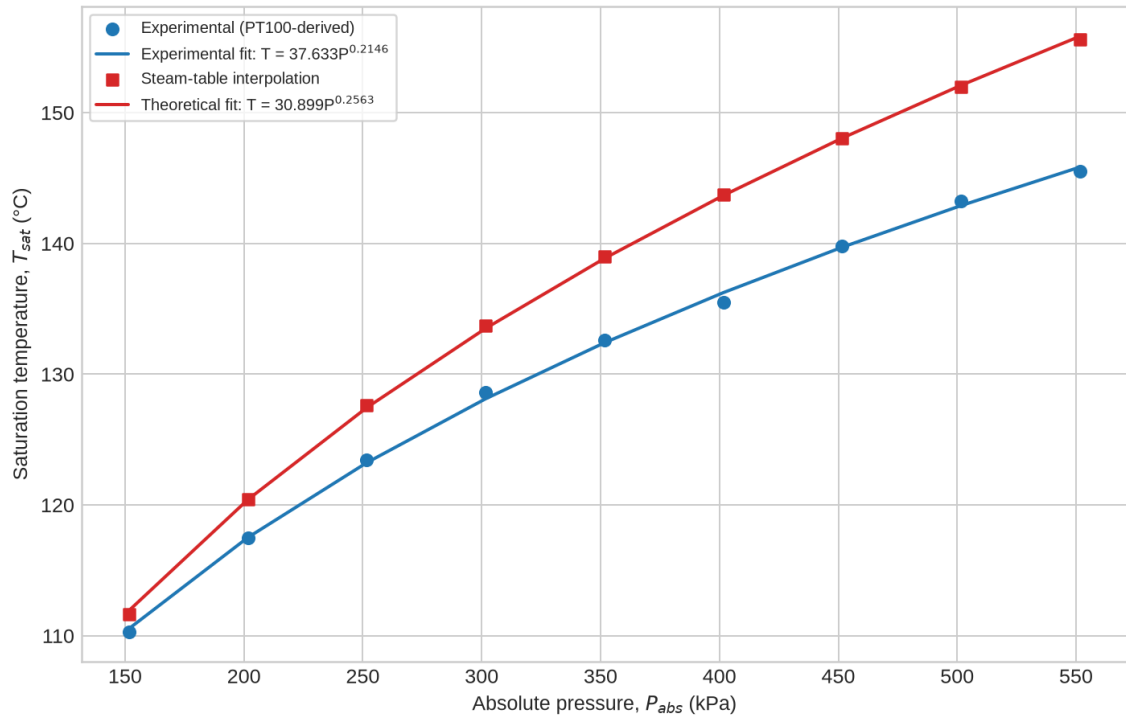
Figure 2: Experimental PT100-derived temperature and interpolated steam-table saturation temperature plotted against absolute pressure, with power-law trendlines.
