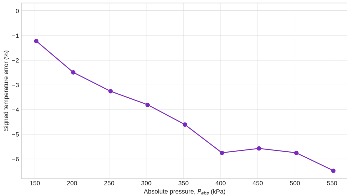
Figure 3: Signed experimental temperature error relative to the interpolated saturated-water values.
